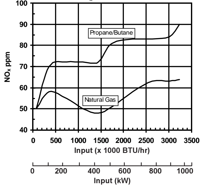
NO x Emission Data
