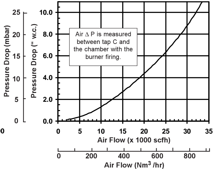
Air Δ P vs. Air Flow
