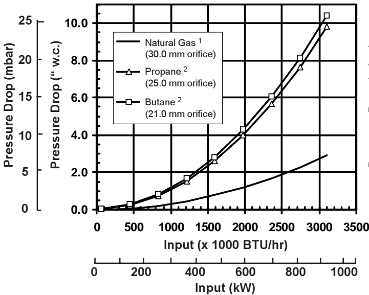
Fuel Orifice Δ P vs. Input
